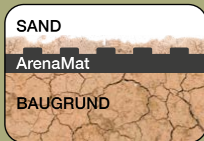
2-Schicht-System
